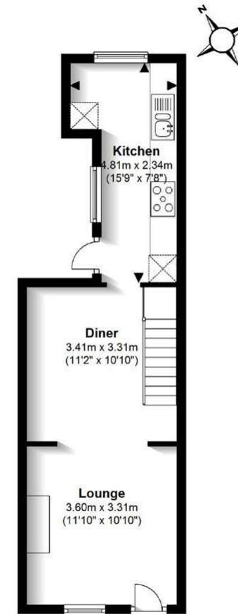
Ground Floor Approx. 31.7 sq. metres (341.0 sq. feet)
